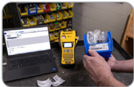
Desktop software
